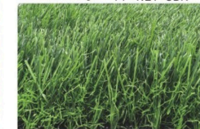
SHA-23422 Type: DQ65-3815 Pile height: 40 mm Stitch Rate: 15 /10cm Gauge: 3/8 inch Density: 15750 stitches/m 2 Dtex: 6500 Backing: PP+NET+SBR
