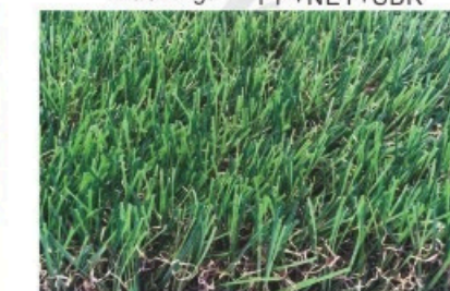
SHA-23416 Type: DQ163-3614 Pile height: 36 mm Stitch Rate: 14 /10cm Gauge: 3/8 inch Density: 14700 stitches/m 2 Dtex: 7200 Backing: PP+NET+SBR
