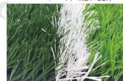
SHA-23417 Type: DSU62-5016 Pile height: 50 mm Stitch Rate: 16 /10cm Gauge: 5/8 inch Density: 10080 stitches/m 2 Dtex: 6200 Backing: PP+NET+SBR
