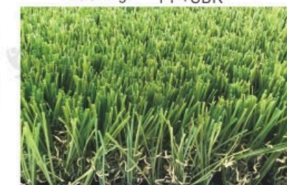
SHA-23415 Type: DQ158-3817 Pile height: 40 mm Stitch Rate: 17 /10cm Gauge: 3/8 inch Density: 17850 stitches/m 2 Dtex: 11500 Backing: PP+PP+SBR(GREEN)
