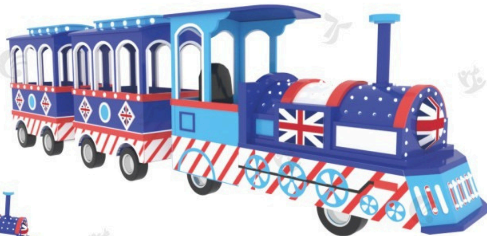
SHA-23424 Locomotive: 238x114x180cm Carriage: 171x114x100cm Capacity: 16 people Voltage: 48V Speed: 7km/h Radius: 5.5 M Volume: 12 m 3
