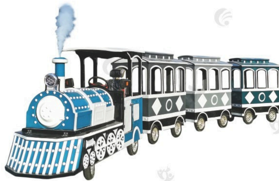
SHA-23423 Locomotive: 270x100x220cm Carriage: 162x100x190cm Capacity: 18 people Voltage: 48V Speed: 7km/h Radius: 6 M Volume: 15 m 3
